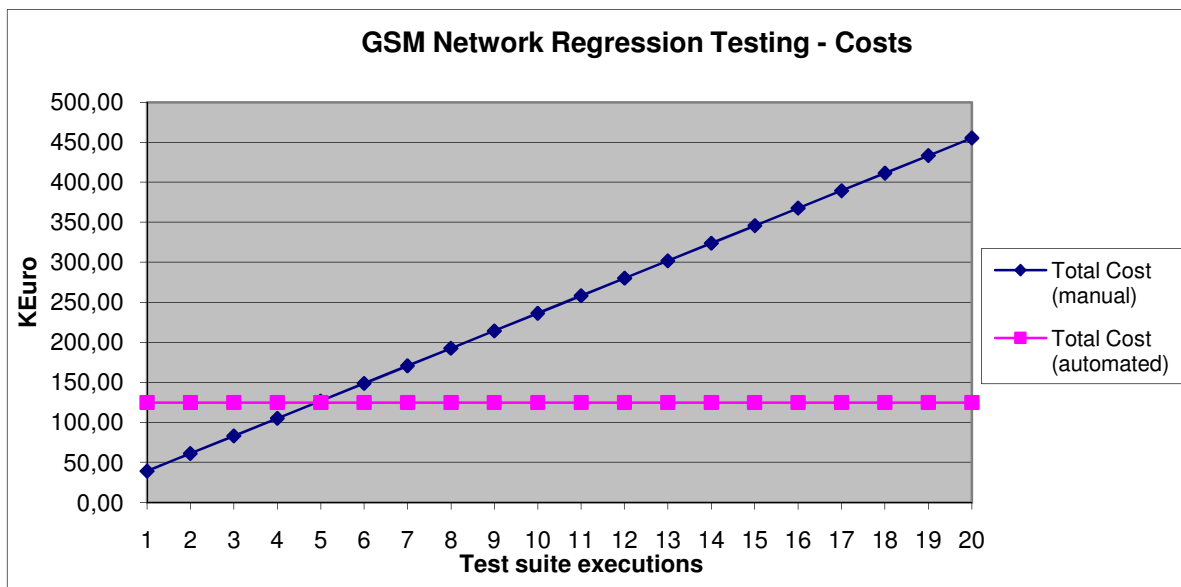
Figure 1: Estimated costs savings for mobile core network regression testing
