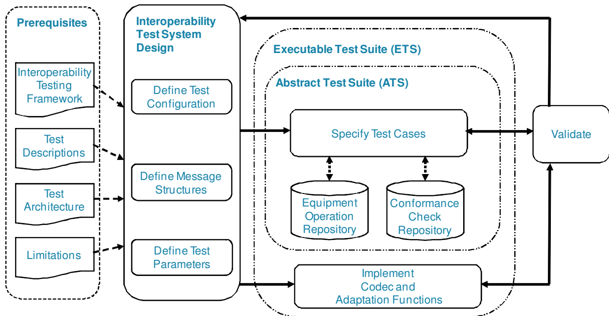
Figure 4: The development process for an interoperability test system
