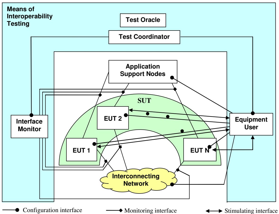
Figure 3: General framework for interoperability testing
