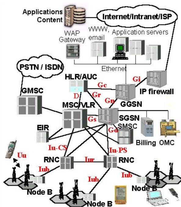
Figure 5: Mobile core network
